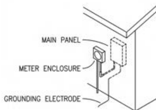
UNDERGROUND ENTRANCE
