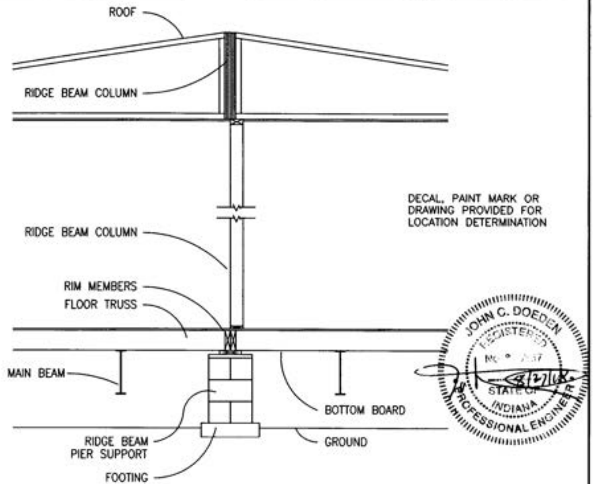
FIGURE 4.4 TYPICAL RIDGE BEAM SUPPORT COLUMN PIER
