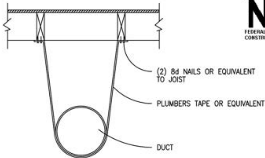
SECTION "A"
