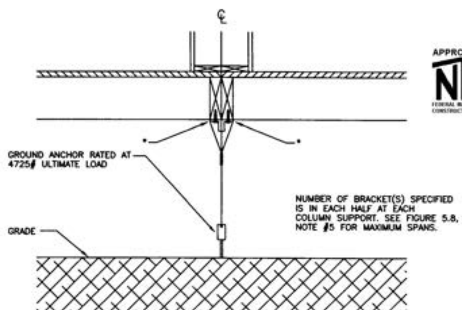
END VIEW
