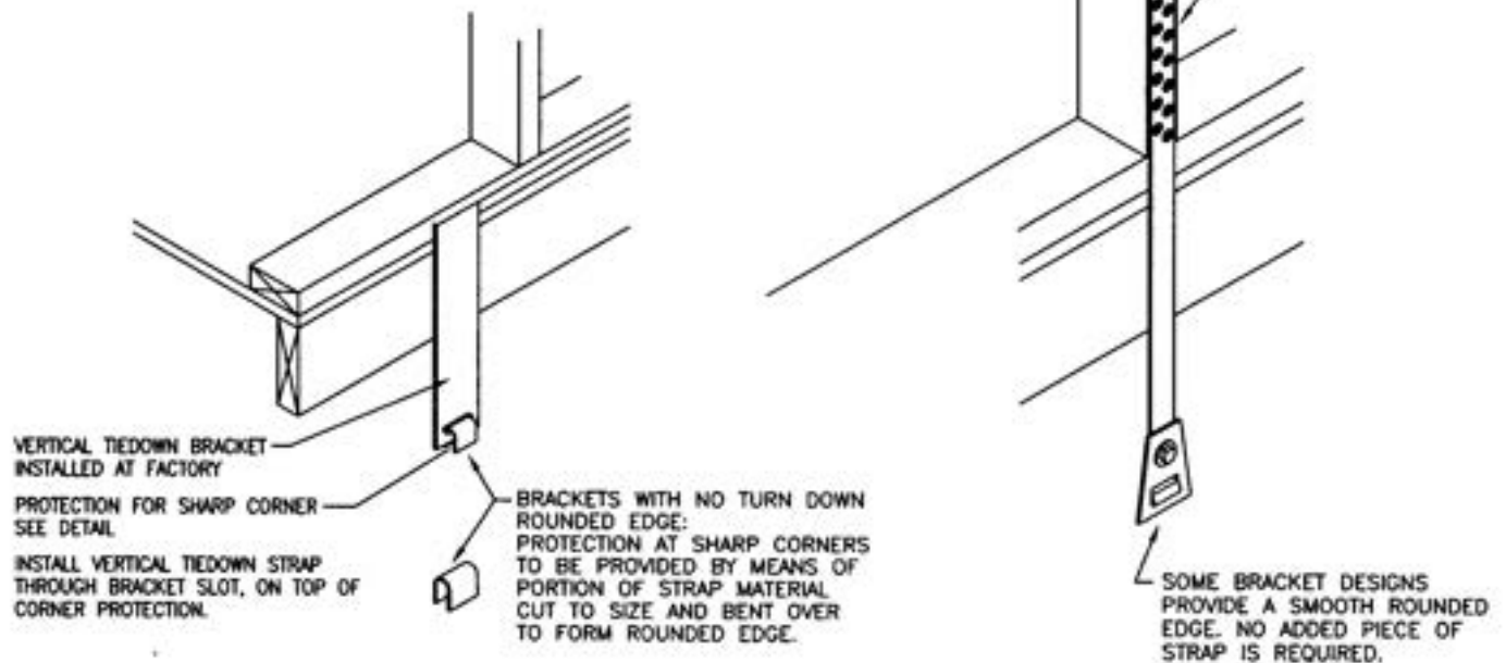
FIGURE 5.15.1 INSTALLATION INSTRUCTIONS ANCHOR STRAP PROTECTION
