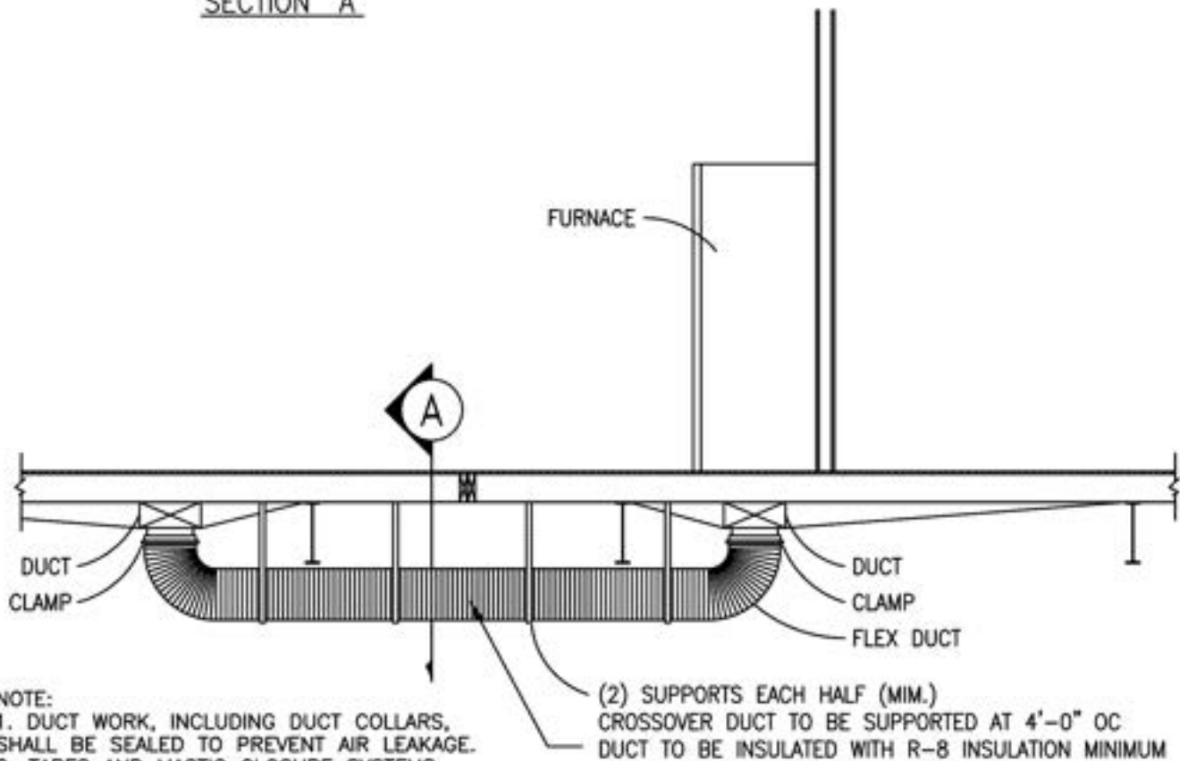
SECTION "A"
