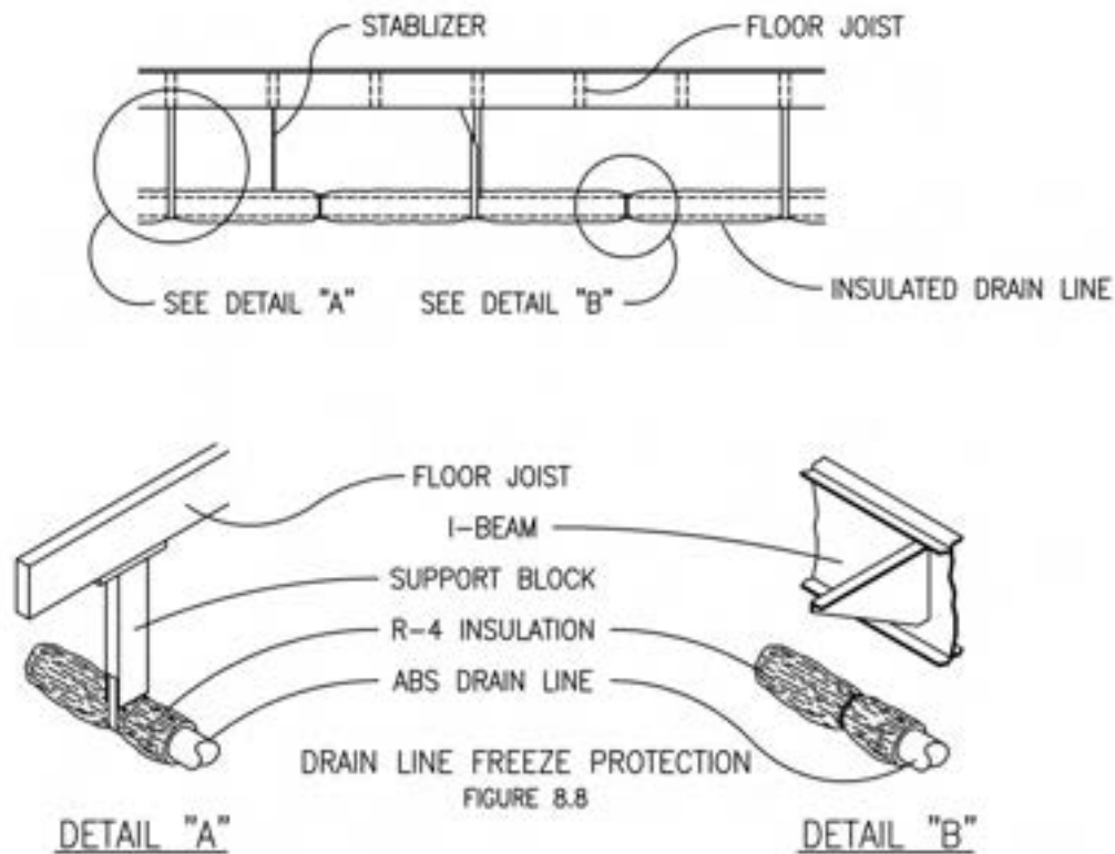
FIGURE 8.6 DRAIN LINE SITE INSTALLATION AND CONNECTION
