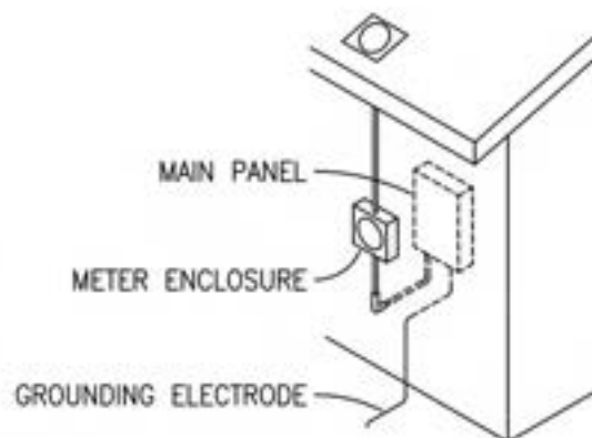
OVERHEAD ENTRANCE
