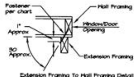
Extension Framing To Wall Framing Detail
